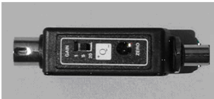
Figure 5 Charge Sensor – measures voltage difference between its red and black leads. Left: Shown attached to the lead assembly. Right: The gain switch (used to amplify small signals) should be set at 1. The zero button sets the output signal to zero.
